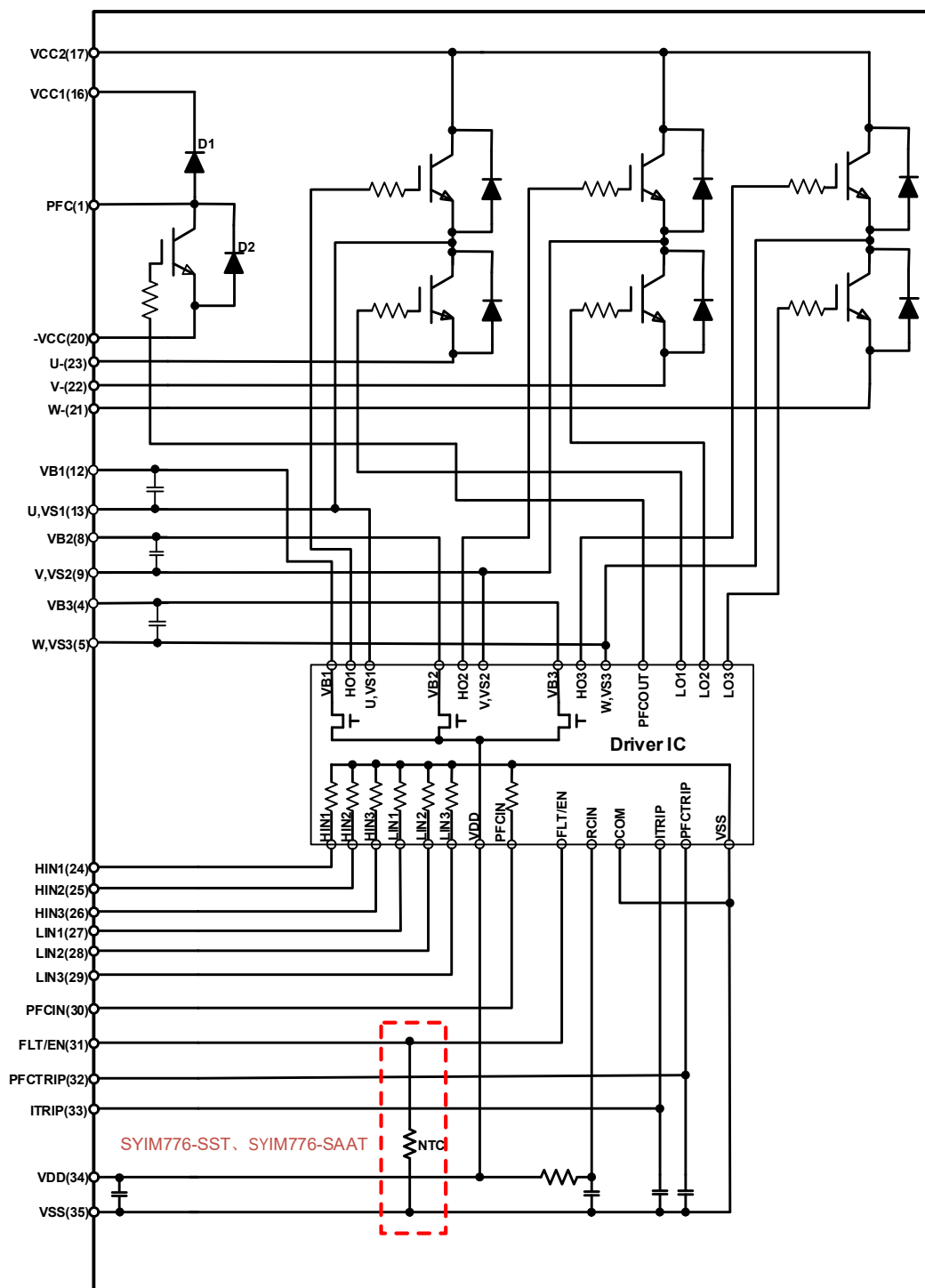
Figure 1 Module Circuit Diagram
