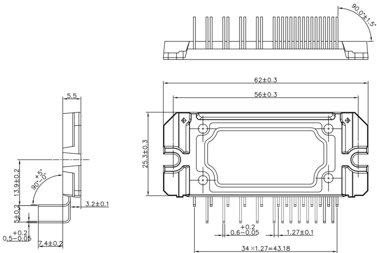
Figure 16 Package Outline
